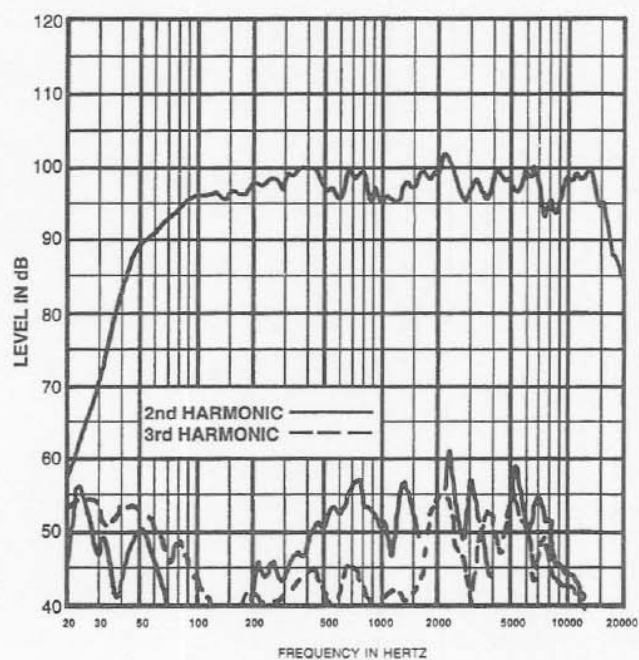
FIGURE 3 UPI-122 Frequency Response (1 watt at 1 meter)
