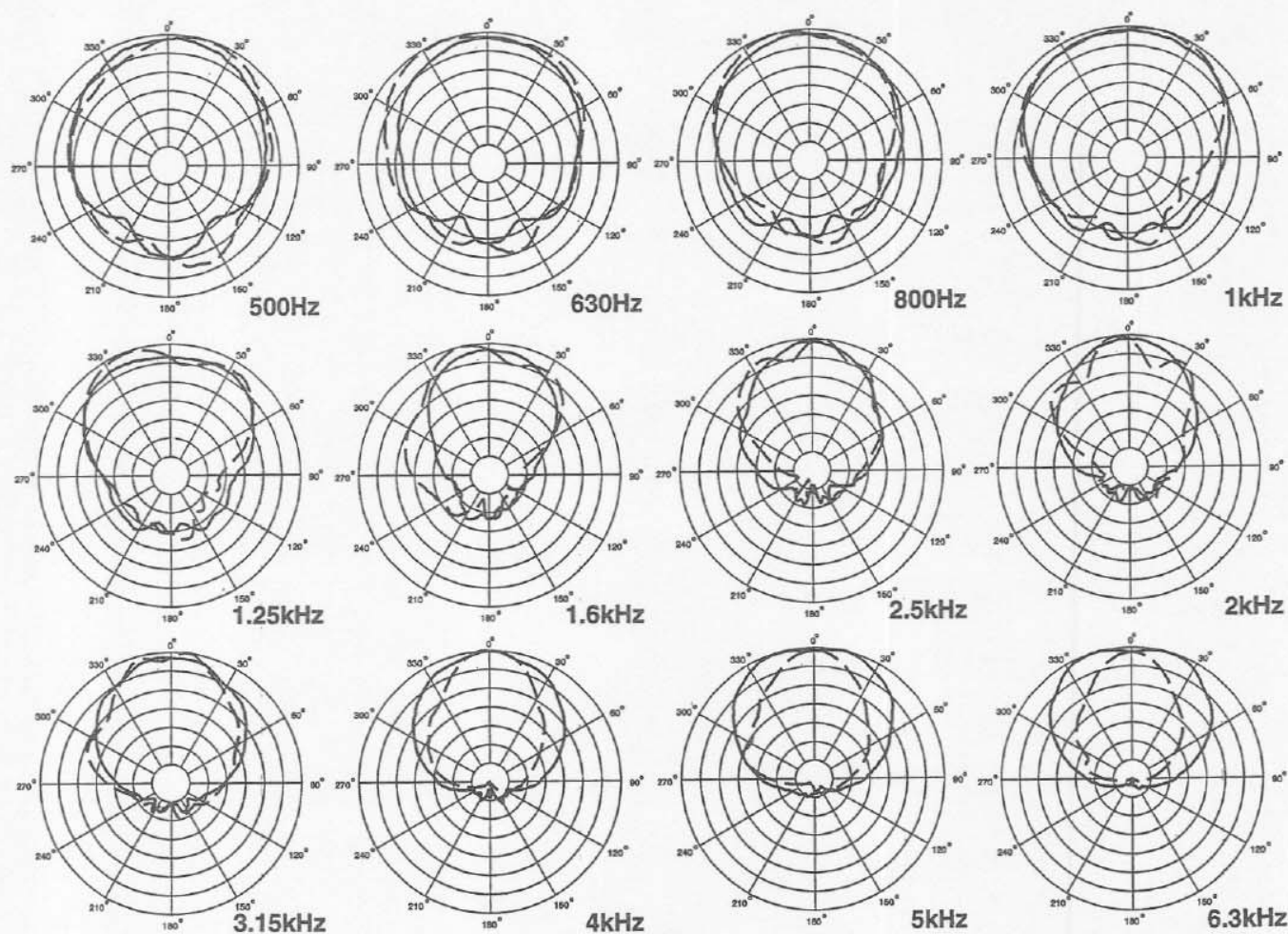
FIGURE 1 UPI-122 Polar Response
